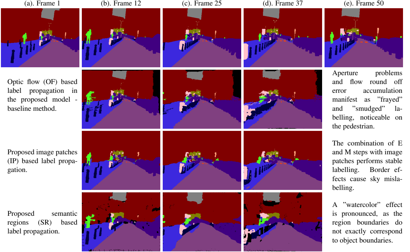
Figure 4. Seq 2 - Frames 1 & 50 on the top row are user provided labels for label propagation. Ground truth for frames 12, 25 & 37 are provided for comparison on the top row. The proposed IP method performs best
